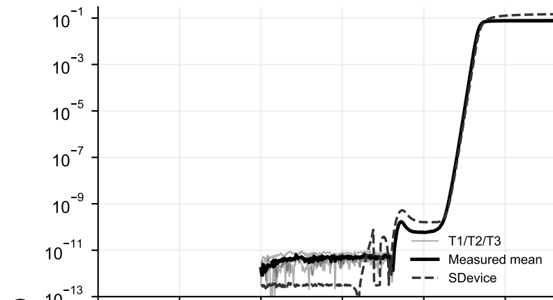
T transfer: measured T1/T2/T3 and mean vs SDevice
