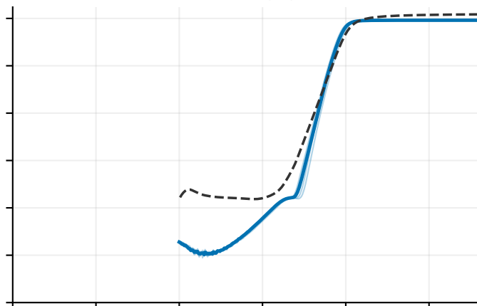
T transfer: measured T1/T2/T3 and mean vs SDevice
