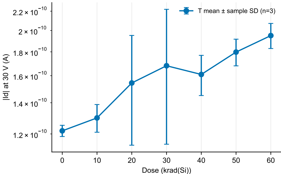
T-only measured |I_d| at 30 V (A) Output, V_{GS} = -20 V
