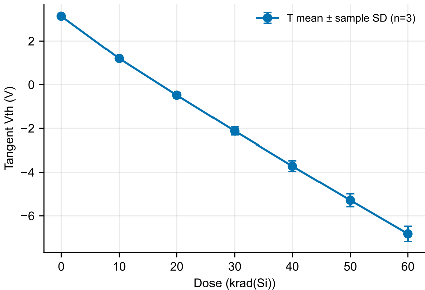
T-only measured Tangent V_{th} (V) Transfer, V_{DS} = 0.1 V
