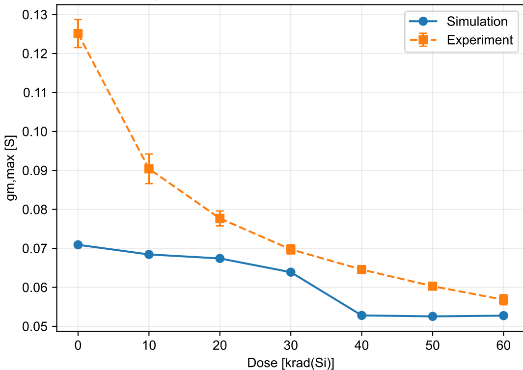
S device gm,max [S]: simulation solid / experiment dashed
