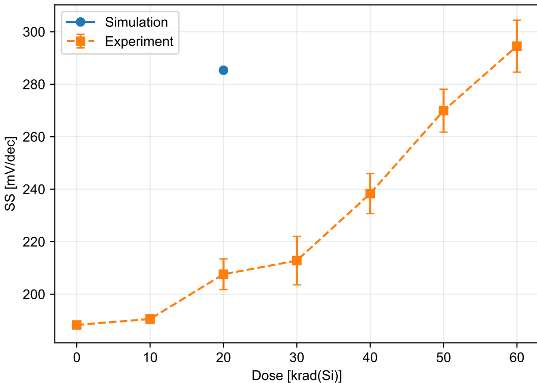
S device SS [mV/dec]: simulation solid / experiment dashed
