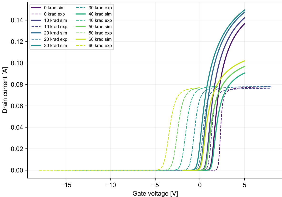
S device transfer: simulation solid / experiment dashed
