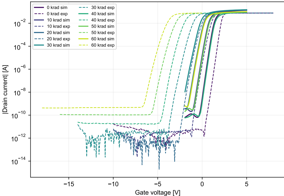
S device transfer: simulation solid / experiment dashed
