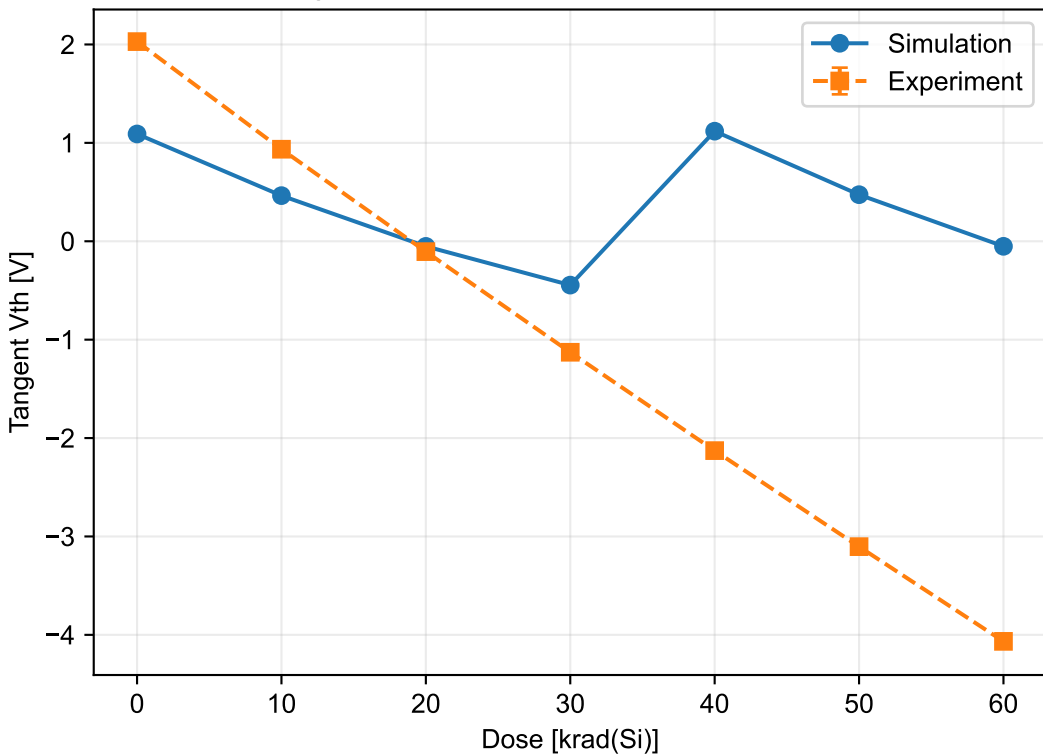
S device Tangent V_{th} [V]: simulation solid / experiment dashed
