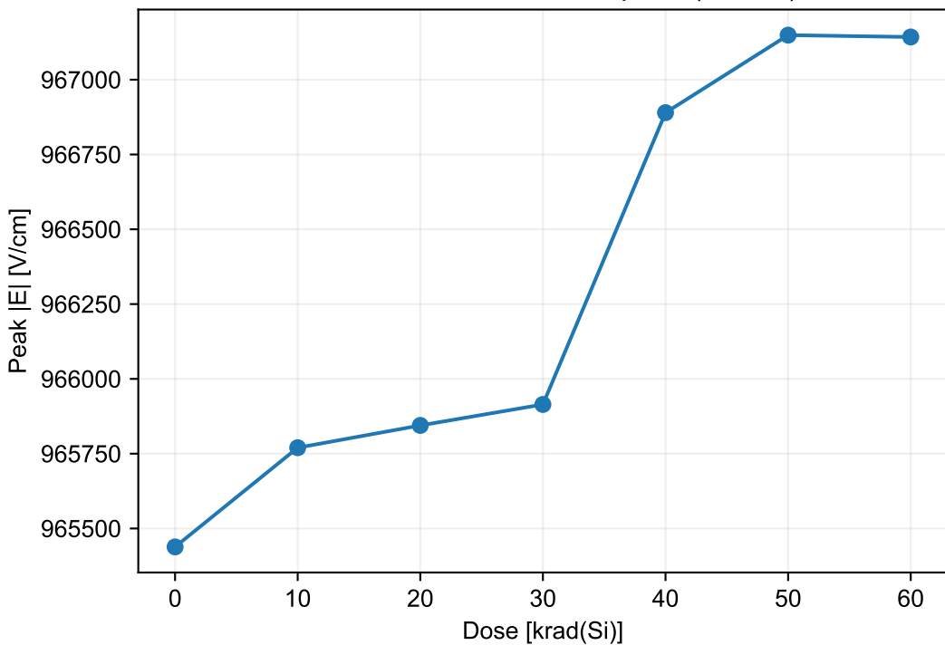
Fixed-Y transfer-end field peak (not BV)
