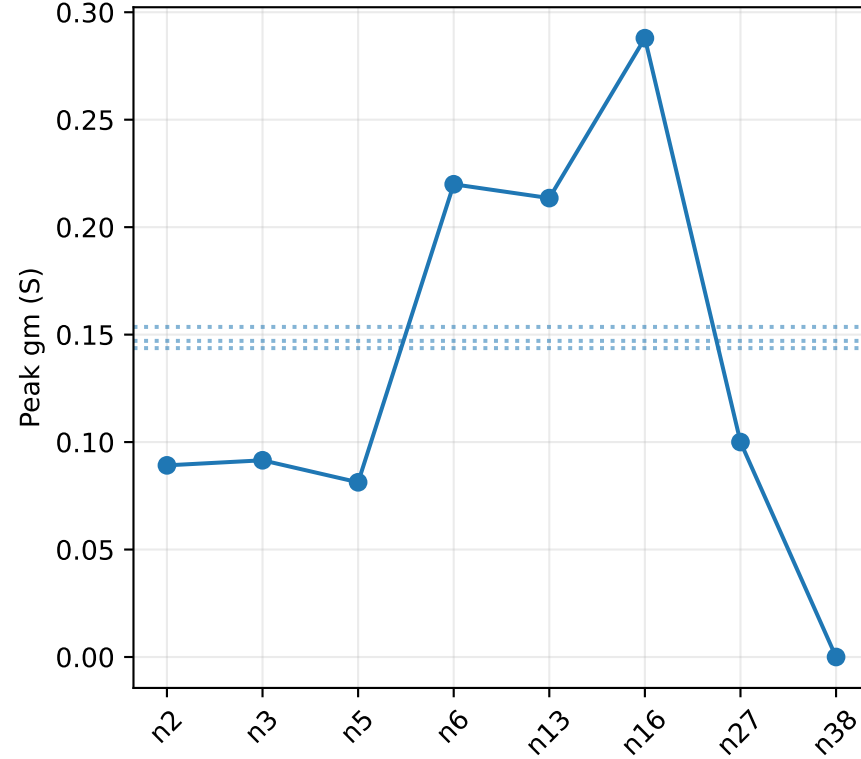
S transfer metrics using analysis_config algorithms Historical exploratory data / formal_valid=false; measured filter device_group=S, scan_no=1
