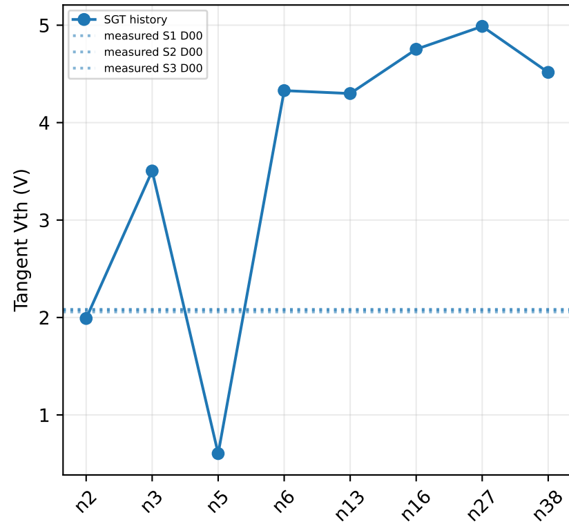
S transfer metrics using analysis_config algorithms Historical exploratory data / formal_valid=false; measured filter device_group=S, scan_no=1
