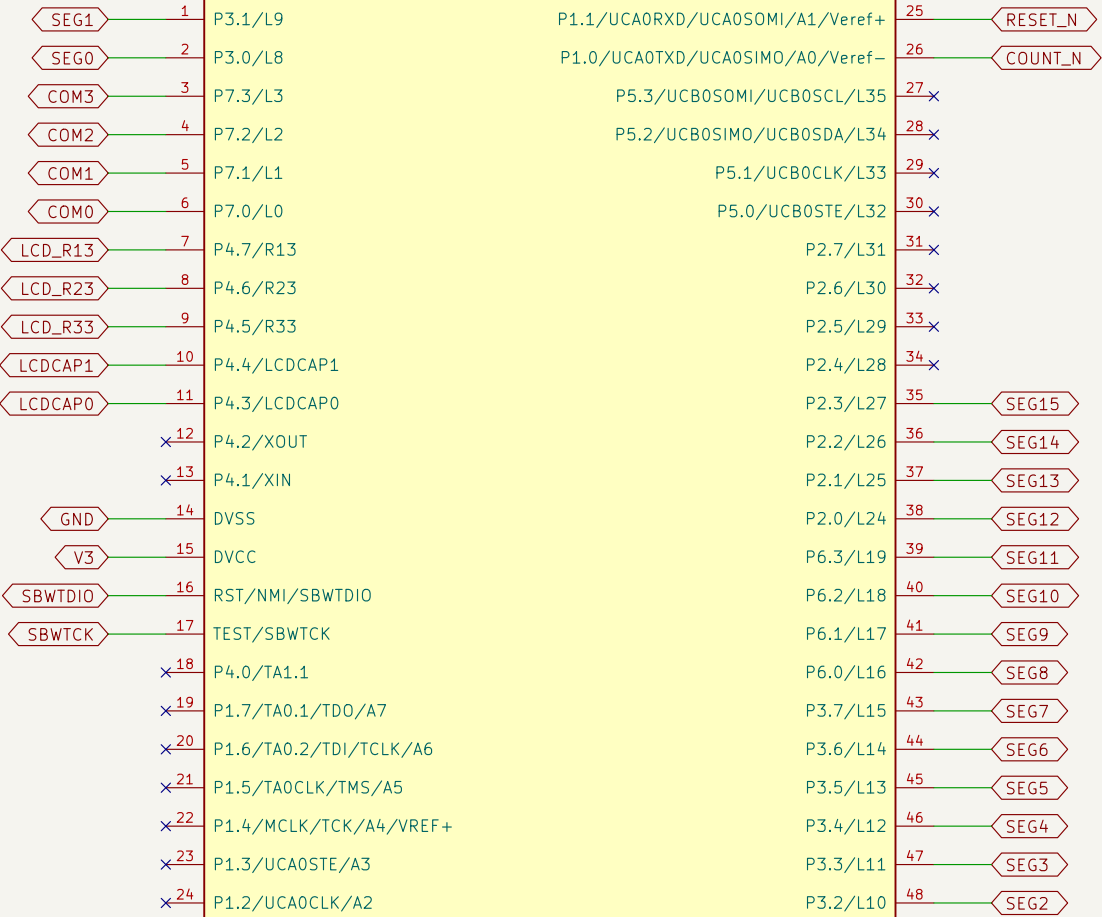
U1 MSP430FR4133IG48R
