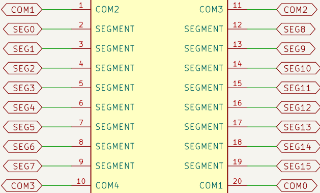
DS1 DE188-RU-30/7.5/V(3V)
