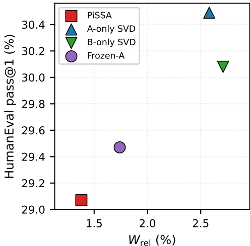
(a) Math: anchor strength vs reasoning (b) Code: anchor strength vs generation
