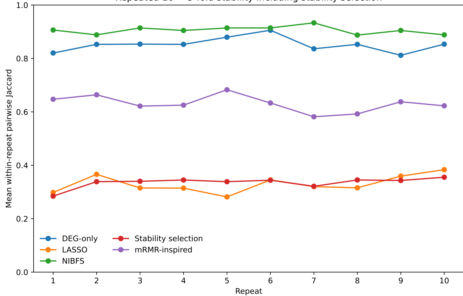
Repeated 10 × 5-fold stability including stability selection
