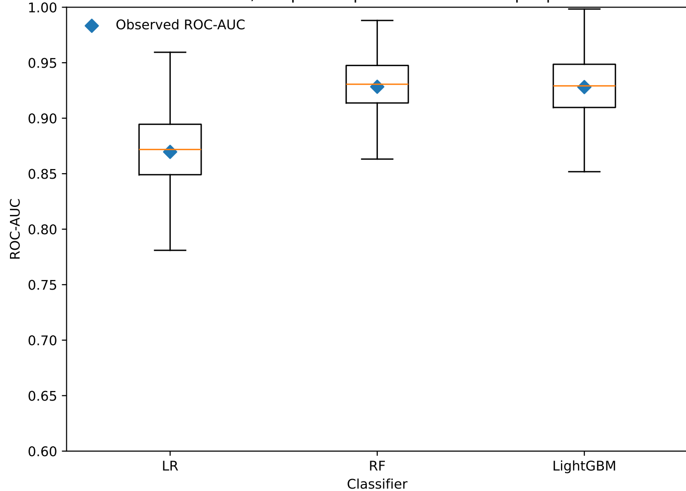
GSE15852: 2,000 patient-pair cluster-bootstrap replicates
