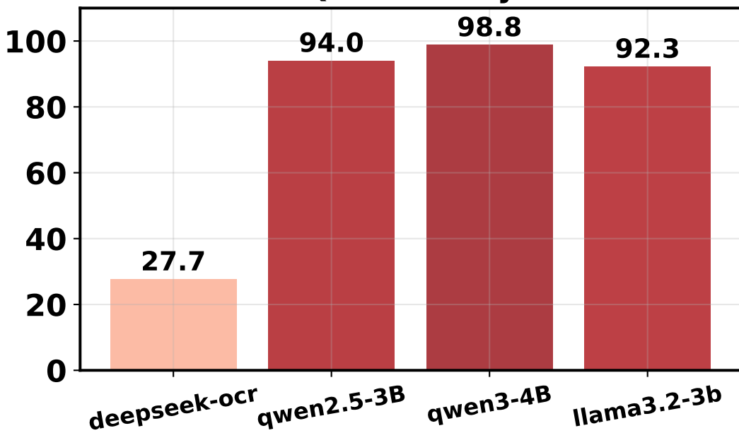
QA Accuracy
