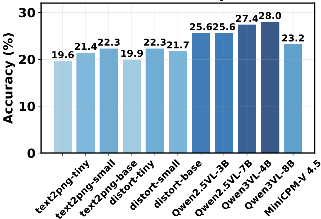
VQA Accuracy
