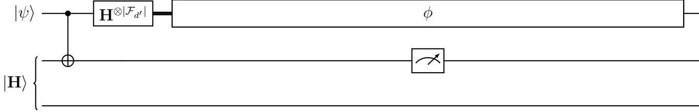
Figure 10: Gate teleportation of the Hadamard gate, using the resource |\mathbf{H}\rangle . We emphasize that although the Hadamard (at least Hadamard-type) has an O(1) -depth gate realization (at least when d' = d/2 ), we still need all the operations on the quantum register to be strictly transversal for the sake of the proof. Thus, we realize the Hadamard via gate teleportation.
