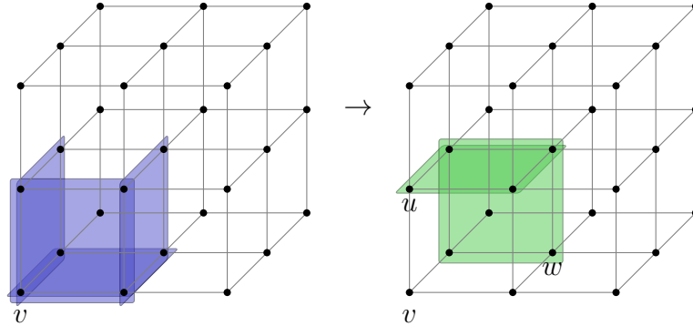
Figure 6: Consider the (3,2) -Toric code, with qubits and X -checks set on the 2- and 1-dimensional faces. In blue, we have a 2-dimensional chain where the vertex achieving the maximum of L_{d+1} , denoted by v , does not see any unsatisfied checks in its positive local view. The green faces represent a 2-dimensional chain, which is the reduced form of the blue. In particular, any local maximum of L_{d+1} (vertices u and w ) sees a non-trivial syndrome in its positive local view. Namely, the maximal points of L_{d+1} in the chain are also the maximal points in the boundary \partial^- .
