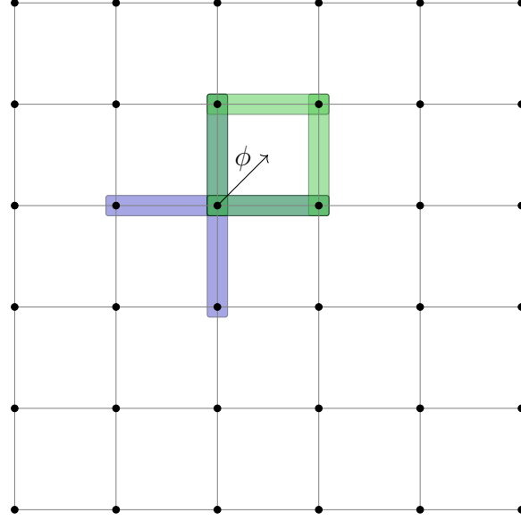
Figure 8: An outline of Example 4.39. The \phi -transpose sends Z -stabilizers to X -stabilizers and vice versa. Here we consider the (2, 1) Toric code; namely, the Z -stabilizers (parity checks) are set on the vertices, and the X -stabilizers (phase checks) are set on the squares. In blue and green, we have the edges corresponding to checks \partial^+ \theta_{(2,3),\{\}}^{\cdot} and \partial^- \theta_{(2,3),\{(0,1),(1,0)\}}^{\cdot} . The example shows that indeed \phi maps between the two.
