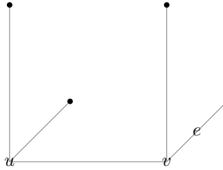
Figure 2: SWEEP rule
