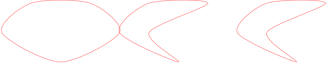
Figure 5: On the left is the Toric Graph. On the right are cross and face checks.
