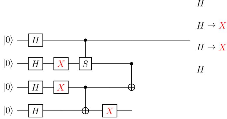
Figure 1: Example of a subjected quantum circuit: the even layers (0, 2, 4) contain the original gates, while the faults are imposed on the odd layers and marked in red.
