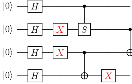
Figure 1: Example of a subjected quantum circuit: the even layers (0, 2, 4) contain the original gates, while the faults are imposed on the odd layers and marked in red.
