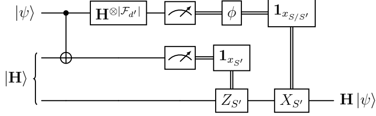
Figure 10: Gate teleportation of the Hadamard gate, using the resource |\mathbf{H}\rangle . We emphasize that although the Hadamard (at least Hadamard-type) has an O(1) -depth gate realization (at least when d' = d/2 ), we still need all the operations on the quantum register to be strictly transversal for the sake of the proof. Thus, we realize the Hadamard via gate teleportation.
