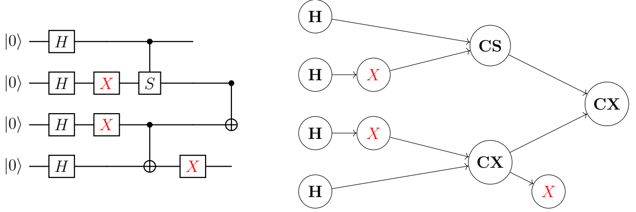
Figure 1: Example of a subjected quantum circuit: the even layers (0, 2, 4) contain the original gates, while the faults are imposed on the odd layers and marked in red.
