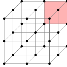
Figure 1: SWEEP rule
