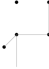
Figure 2: SWEEP rule
