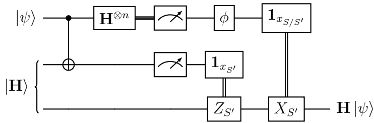
Figure 9: Gate teleportation of the Hadamard gate, using the resource |\mathbf{H}\rangle . We emphasize again that although the Hadamard (at least Hadamard-type) has an O(1) -depth gate realization (at least when d' = d/2 ), we still need all the operations on the quantum register to be strictly transversal for the sake of the proof. Thus, we realize the Hadamard via gate teleportation.
