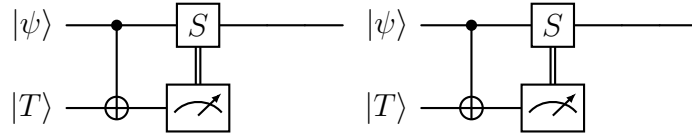
Figure 8: Simulating the T -gate, using the |T\rangle magic state.
