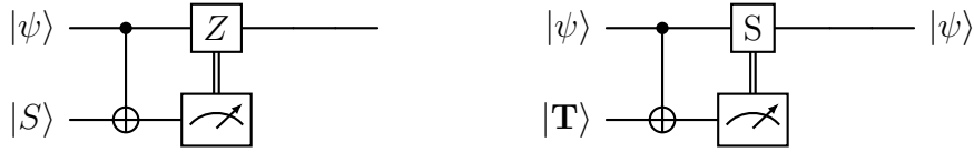
Figure 8: Simulating the T -gate, using the |T\rangle magic state.
