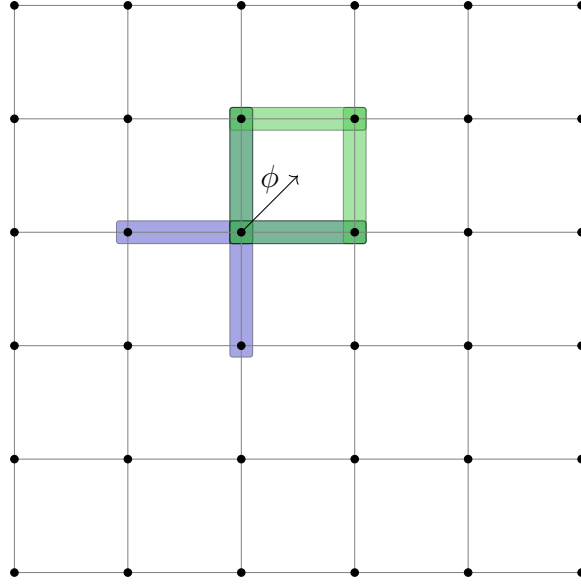
Figure 8: An outline of Example 4.40. The \phi -transpose sends Z -stabilizers to X -stabilizers and vice versa. Here we consider the (2, 1) Toric code; namely, the Z -stabilizers (parity checks) are set on the vertices, and the X -stabilizers (phase checks) are set on the squares. In blue and green, we have the edges corresponding to checks \partial^+ \theta_{(\mathbf{2}, \mathbf{3}), \{\}}^{\circ} and \partial^- \theta_{(\mathbf{2}, \mathbf{3}), \{(0,1), (1,0)\}}^{\circ} . The example shows that indeed \phi maps between the two.
