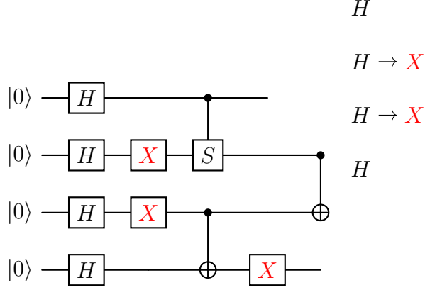
Figure 1: Example of a subjected quantum circuit: the even layers (0, 2, 4) contain the original gates, while the faults are imposed on the odd layers and marked in red.
