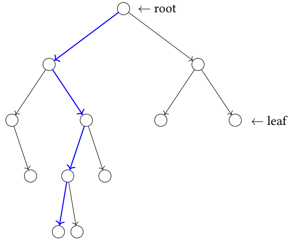
Algorithm 1: Investigation
