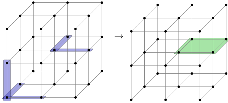
Figure 4: SWEEP rule
