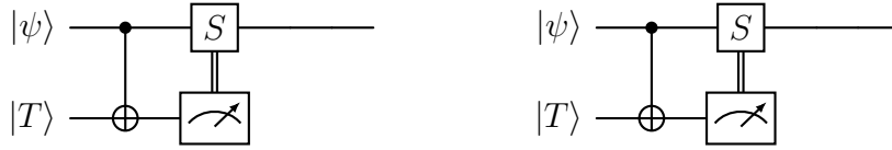
Figure 8: Simulating the T -gate, using the |T\rangle magic state.
