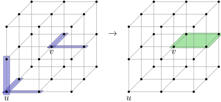
Figure 6: An example of applying the sweep rule within the (3, 2) -Toric code. In the (3, 2) -Toric code, bits are placed on the squares and Z -stabilizers (parity checks) on the edges. The view is restricted to two vertices, u and v . On the left, the unsatisfied positive checks of u and v are highlighted in blue. On the right, the bits to be flipped are marked in green. Given the syndrome, vertex v flips one of its positive faces, whereas for u , there is no subset of positive faces that, when flipped, decreases the number of local unsatisfied checks. Therefore, u flips no bit.
