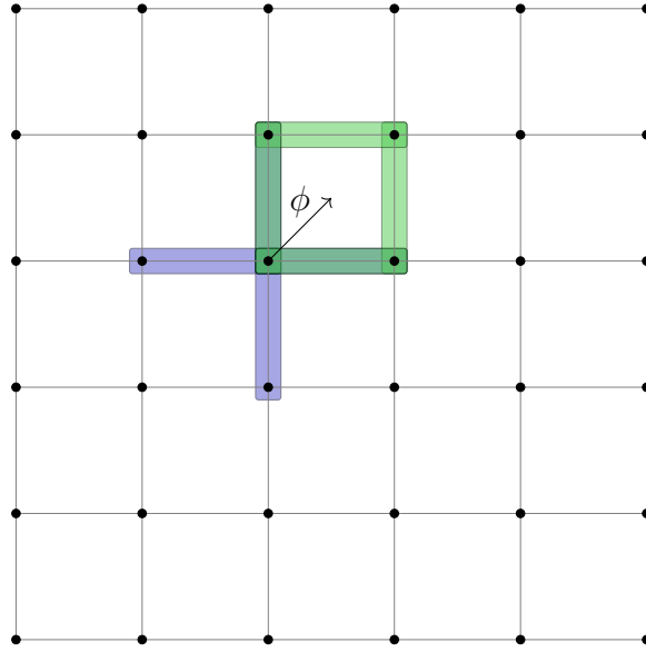
Figure 7: An outline of Example 4.14. The \phi -transpose sends Z -stabilizers to X -stabilizers and vice versa. Here we consider the (2, 1) Toric code; namely, the Z -stabilizers (parity checks) are set on the vertices, and the X -stabilizers (phase checks) are set on the squares. In blue and green, we have the edges corresponding to checks \partial^+ \theta_{(\mathbf{2}, \mathbf{3}), \{\}}^ and \partial^- \theta_{(\mathbf{2}, \mathbf{3}), \{(0,1), (1,0)\}}^ . The example shows that indeed \phi maps between the two.
