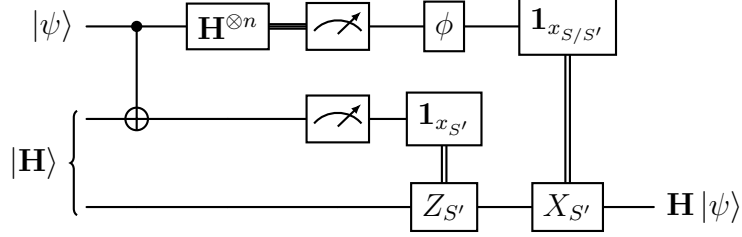
Figure 9: Gate teleportation of the Hadamard gate, using the resource |\mathbf{H}\rangle . We emphasize again that although the Hadamard (at least Hadamard-type) has an O(1) -depth gate realization (at least when d' = d/2 ), we still need all the operations on the quantum register to be strictly transversal for the sake of the proof. Thus, we realize the Hadamard via gate teleportation.
