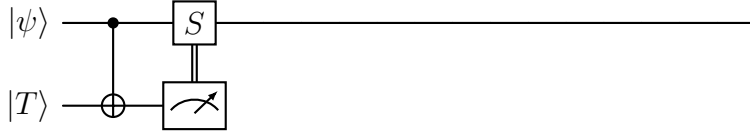
Figure 1: Simulating the T -gate, using the |T\rangle magic state.
