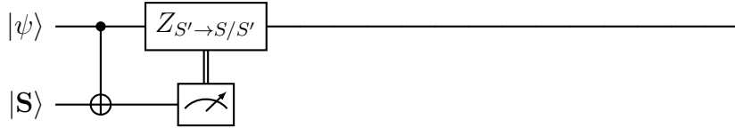
Figure 1: Simulating the \mathbf{S} -gate, using the |\mathbf{S}\rangle magic state.
