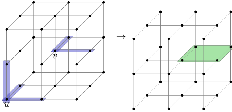
Figure 4: SWEEP rule
