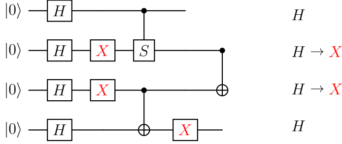
Figure 1: Example of a subjected quantum circuit: the even layers (0, 2, 4) contain the original gates, while the faults are imposed on the odd layers and marked in red.
