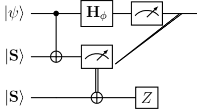
Figure 9: Simulating the \mathbf{S} and \mathbf{T} gates, using the |\mathbf{S}\rangle, |\mathbf{T}\rangle magic states.
