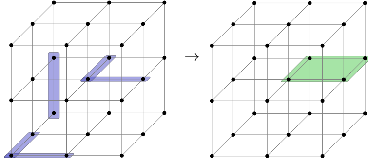
Figure 4: SWEEP rule
