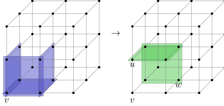
Figure 6: Consider the (3, 2) -Toric code, with qubits and X -checks set on the 2- and 1-dimensional faces. In blue, we have a 2-dimensional chain where the vertex achieving the minimum of L_{d+1} , denoted by v , does not see any unsatisfied checks in its positive local view. The green faces represent a 2-dimensional chain, which is the reduced form of the blue. In particular, any local maximum of L_{d+1} (vertices u and w ) sees a non-trivial syndrome in its positive local view. Namely, the maximal points of L_{d+1} in the chain are also the maximal points in the boundary \partial^- .
