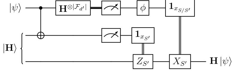
Figure 10: Gate teleportation of the Hadamard gate, using the resource |\mathbf{H}\rangle . We emphasize again that although the Hadamard (at least Hadamard-type) has an O(1) -depth gate realization (at least when d' = d/2 ), we still need all the operations on the quantum register to be strictly transversal for the sake of the proof. Thus, we realize the Hadamard via gate teleportation.
