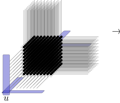
Figure 5: SWEEP rule
