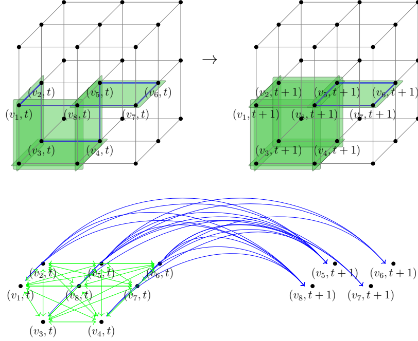
Figure 5: Above: The application of a sweep-cycle, where the green faces represent the bits assignment z , and the blue edges correspond to unsatisfied checks \partial^-z . The vertices in the reduced form are labeled as v_1, v_2, \dots, v_8 . Notice that the leftmost bottom-inner vertex is not in the reduced form even though it belongs to z . Below: The Toom's contour derived from the single computation layer that matches the cycle. Arrows are colored in blue, while forks are colored in green. Note that (v_1, t+1) doesn't belong to the Toom's contour (since v_1 doesn't belong to a reduced error cluster at time t+1 ).
