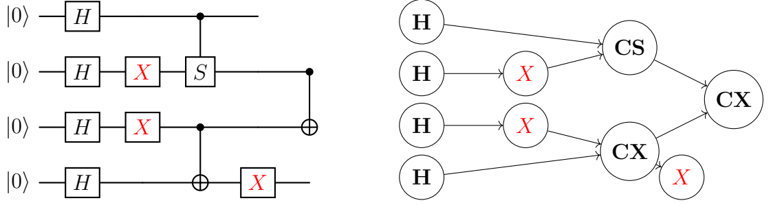
Figure 1: Example of a subjected quantum circuit: the even layers (0, 2, 4) contain the original gates, while the faults are imposed on the odd layers and marked in red.
