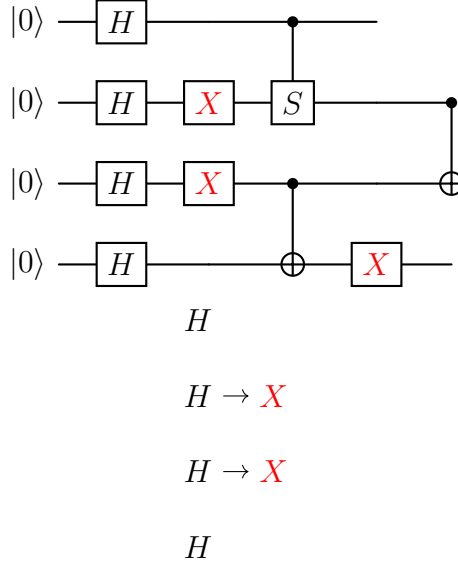
Figure 1: Example of a subjected quantum circuit: the even layers (0, 2, 4) contain the original gates, while the faults are imposed on the odd layers and marked in red.
