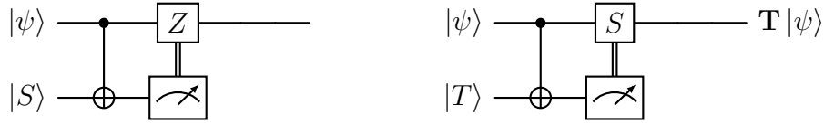
Figure 8: Simulating the T -gate, using the |T\rangle magic state.
