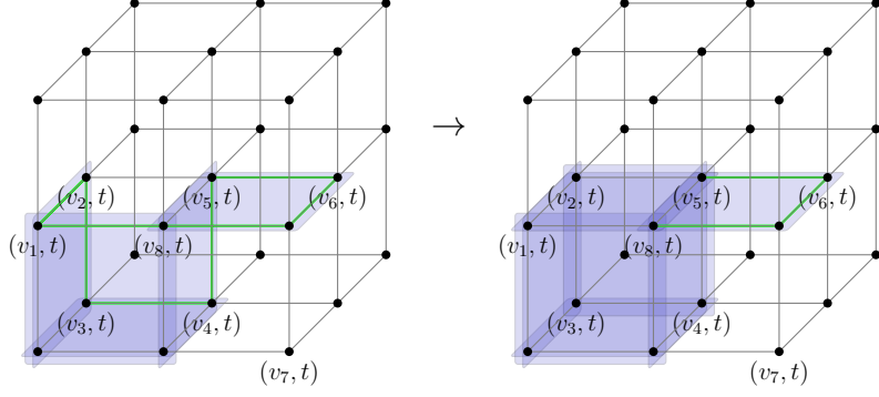
Figure 8: In blue, we have an assignment where the vertex achieving the minimum of L_{d+1} , denoted by v , does not see any unsatisfied checks in its positive local view. The green faces represent an assignment, equivalent to the blue up to stabilizer, such that any local maximum of L_{d+1} (vertices u and w ) sees a non-trivial syndrome in its positive local view.
